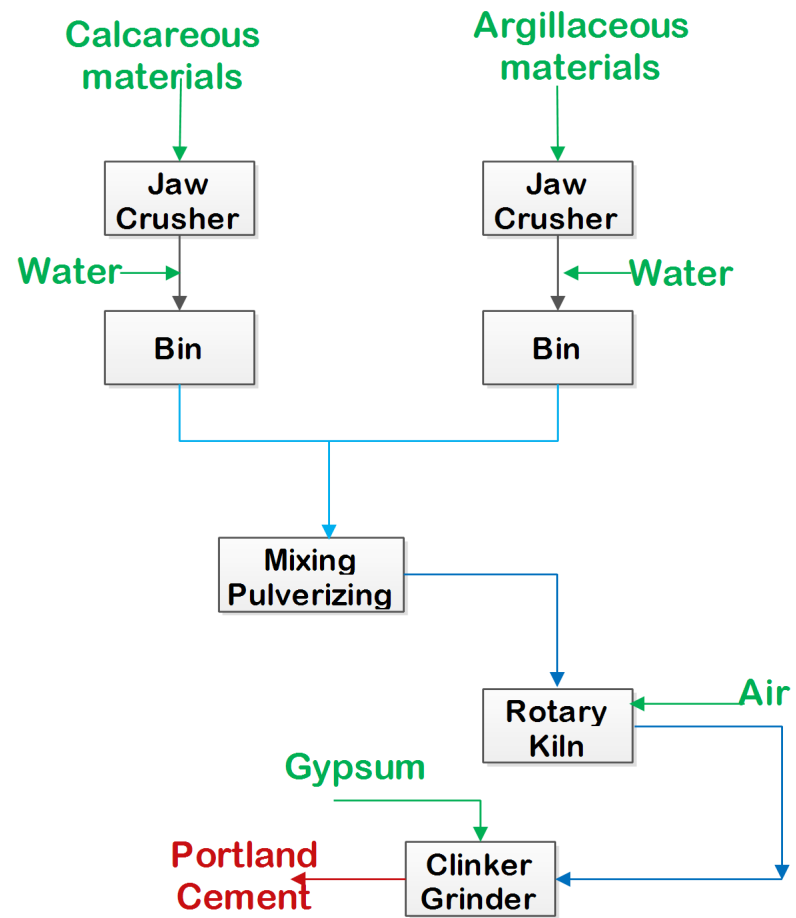
Figure: Manufacturing of Cement by Wet Process
